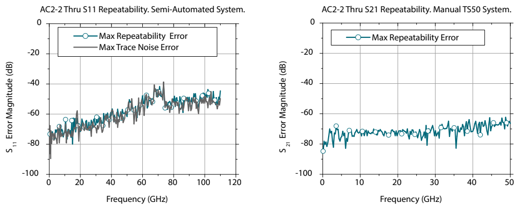
The maximal probe contact repeatability error of the calibrate S11 and S21 of the AC-2 thru standard by T110 and T50 probes.
